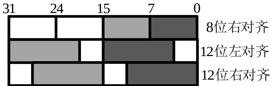
Figure 15-3 Data registers in dual-DAC channel mode
