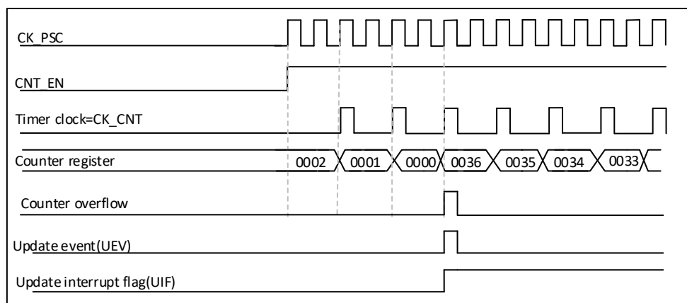
Figure 20-10 Counter timing diagram, internal clock divided by 2
