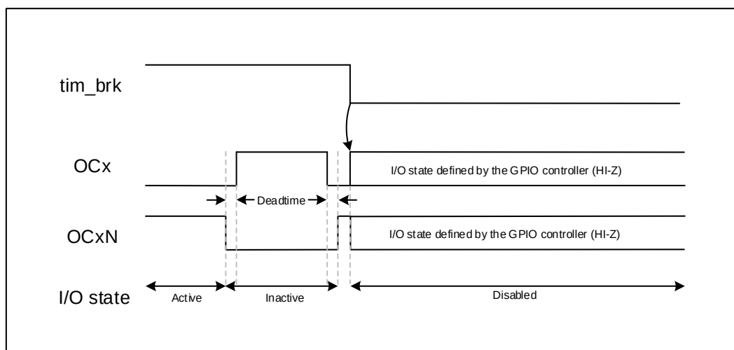
Figure 19-49 PWM output state after braking and braking 2 ( OSSI = 0 )
