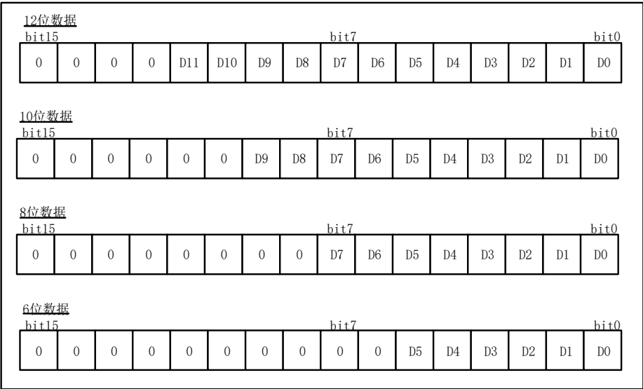
Figure 14-9 right-aligned (offset not enabled, unsigned number)
