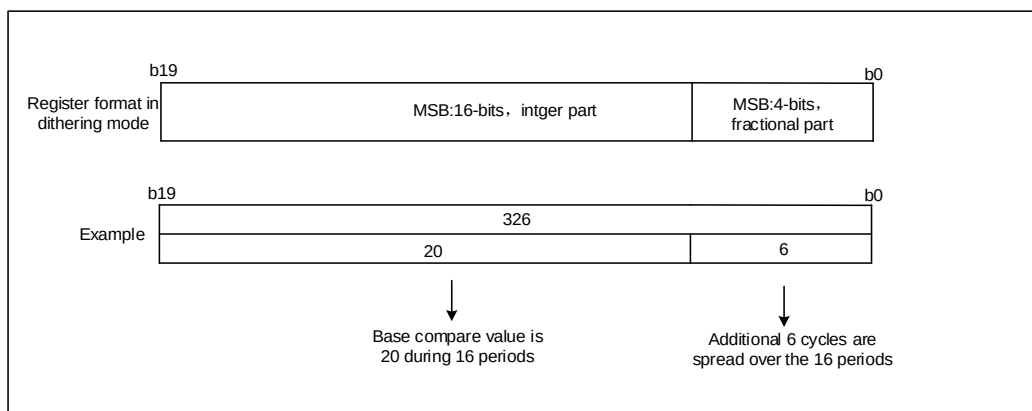
Figure 20-33 Data mapping and register coding in dither mode
