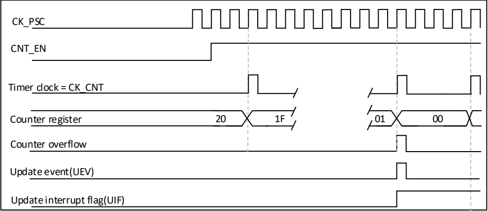
Figure 20-17 Counter timing diagram, internal clock divided by N
