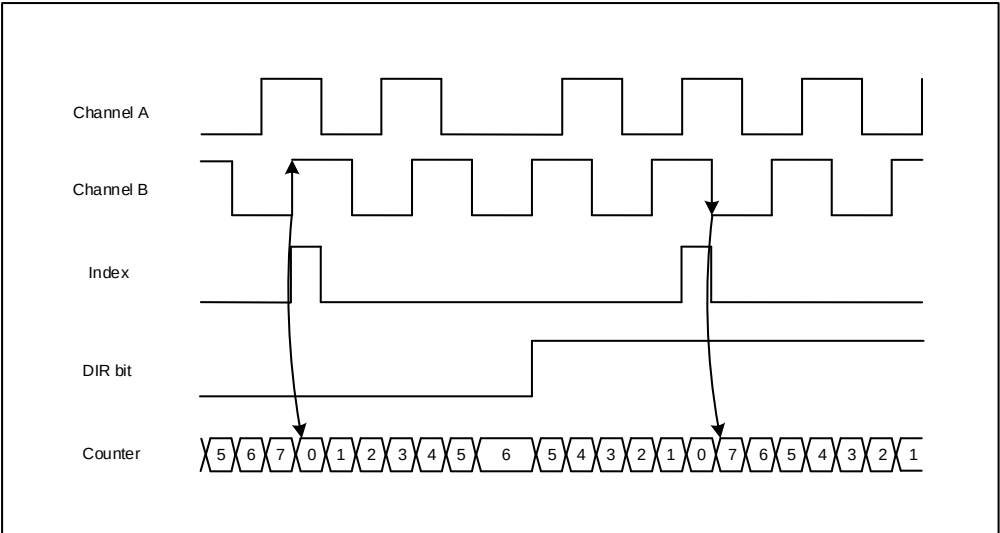
Figure 20-57 indexes and count values when channels A and B are gated
