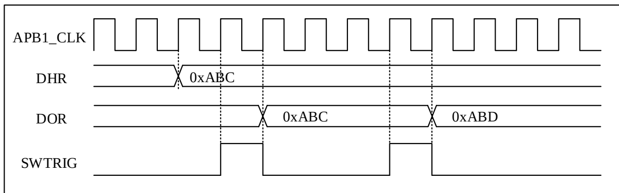
Figure 15-9 DAC conversion with triangulation generation of graphs (software triggered)
