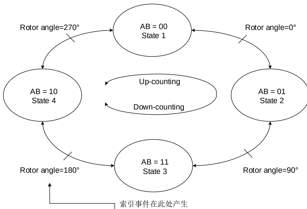
Figure 20-54 Index Generation at IPOS [1: 0] = 11
