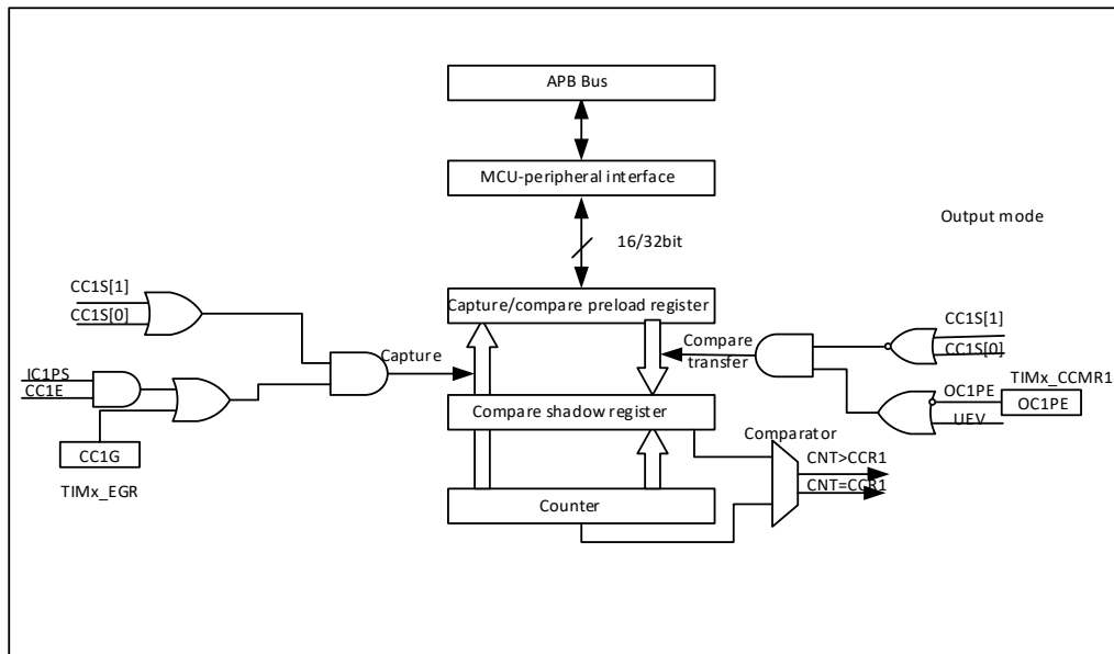
Figure 19-27 Capture/Compare the main circuit of channel 1
