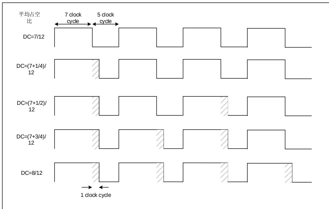
Figure 20-32 jitter principle
