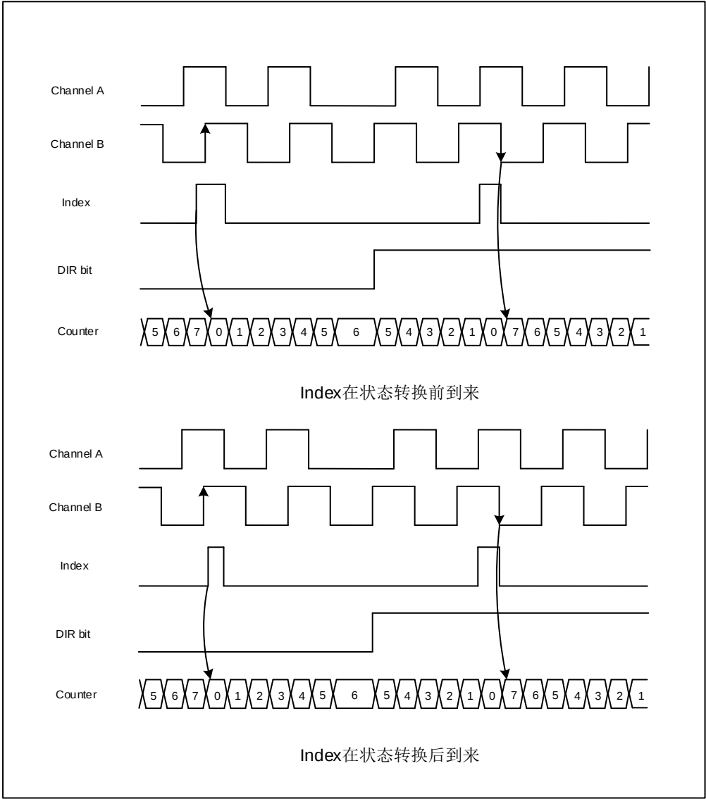
Figure 20-58 Operation of encoder mode with narrow index pulse at IPOS [1: 0] = 11
