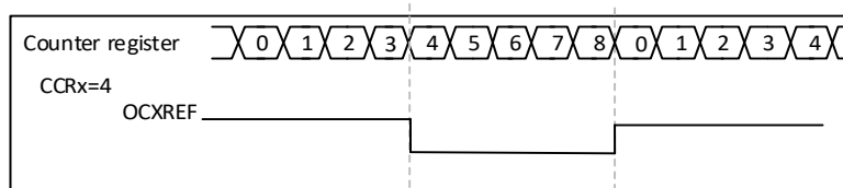
Figure 23-18 Edge-aligned PWM waveforms (ARR=8)
