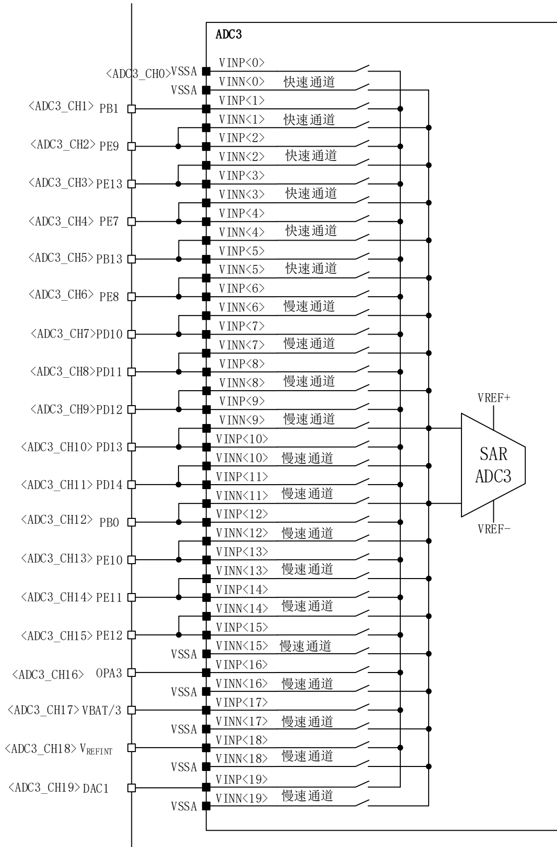
Figure 14-4 ADC3 channel connection relationship
