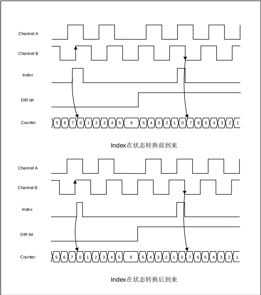
Figure 19-71 Operation of encoder mode with narrow index pulse at IPOS [1: 0] = 11
