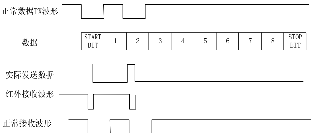
Figure 37-15 IrDA Data Modulation (3/16)-Normal Mode
