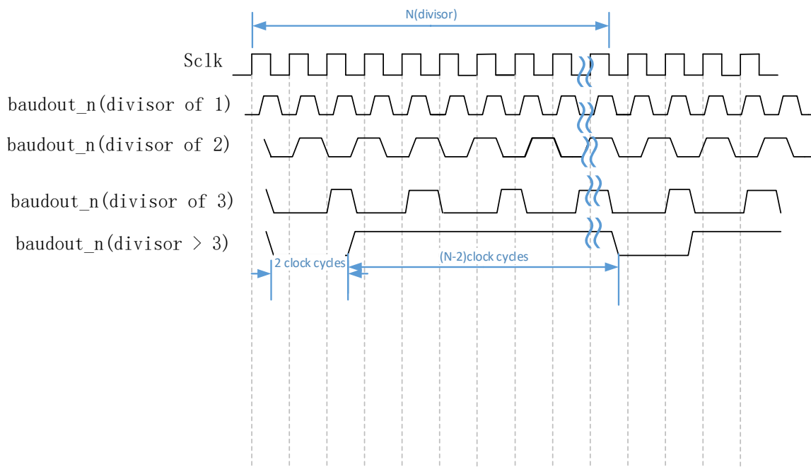
Figure 38-3 timing diagram
