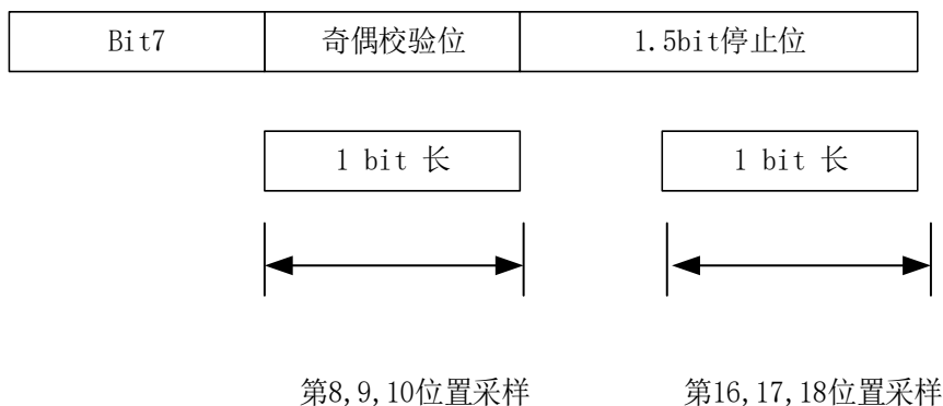
Figure 37-13 1.5 stop bit detection of parity error
