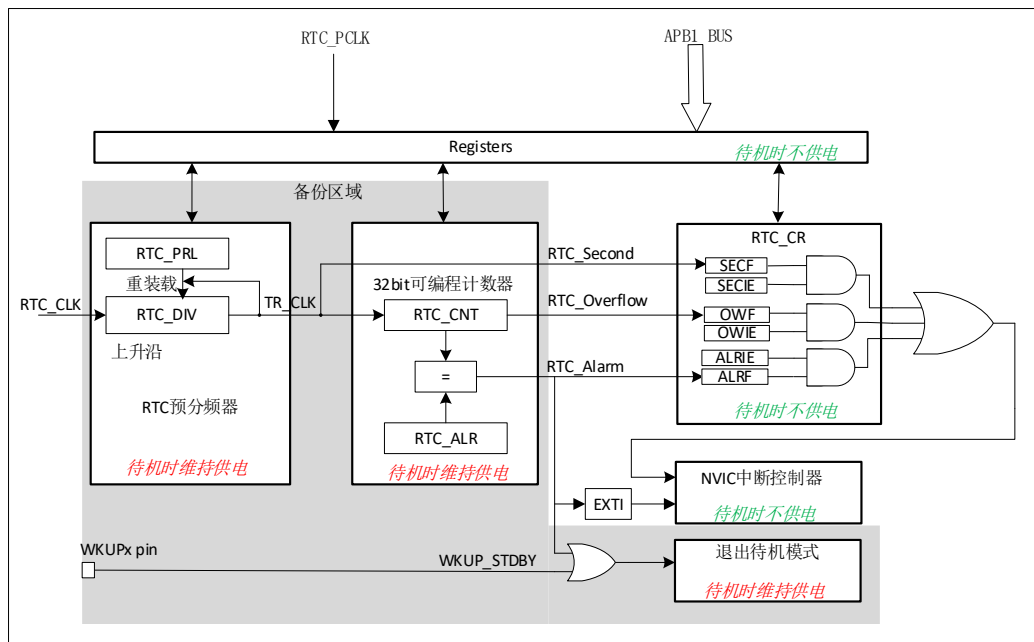
Figure 27-1 RTC functional block diagram
