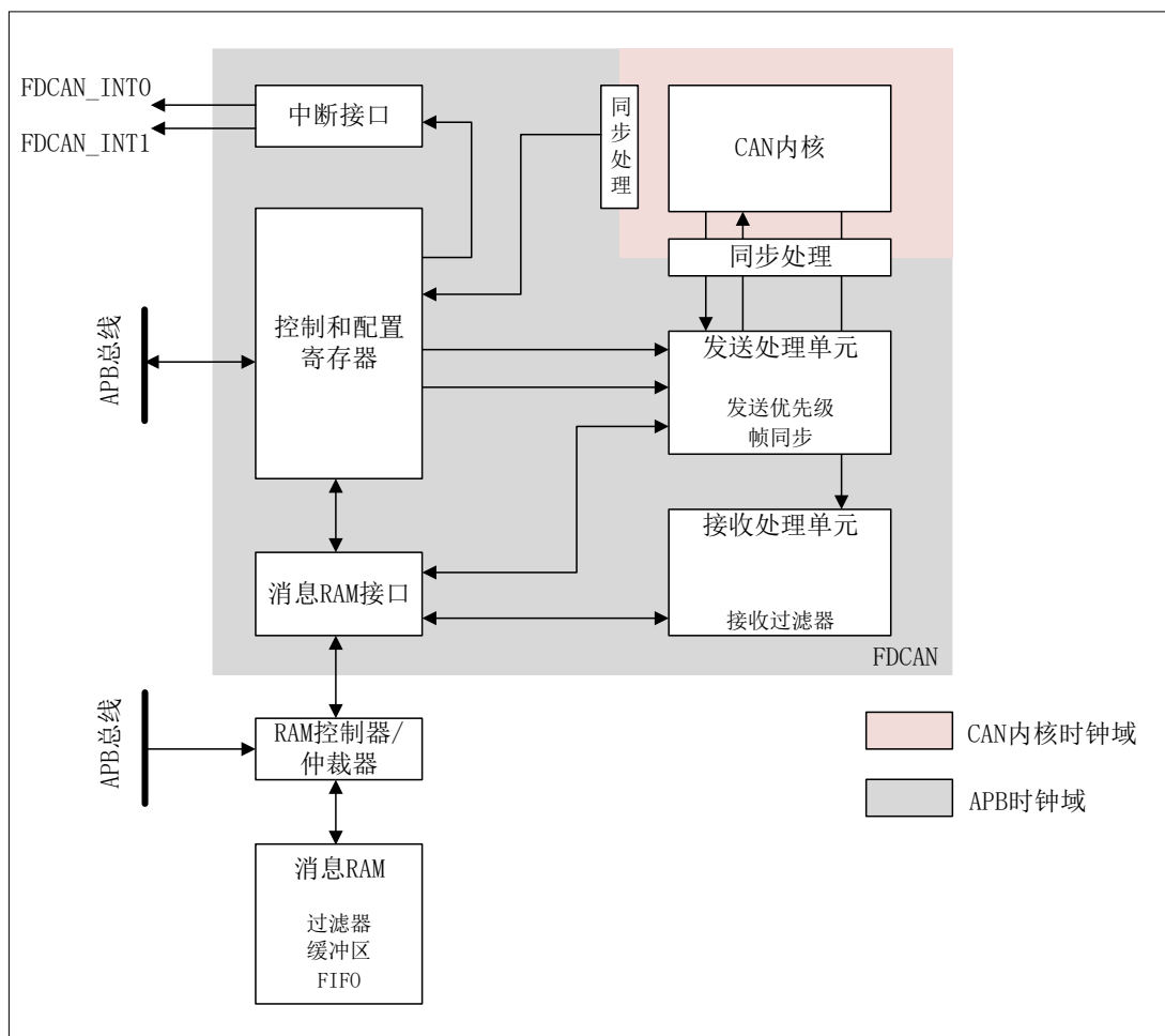
Figure 34-1 Module block diagram
