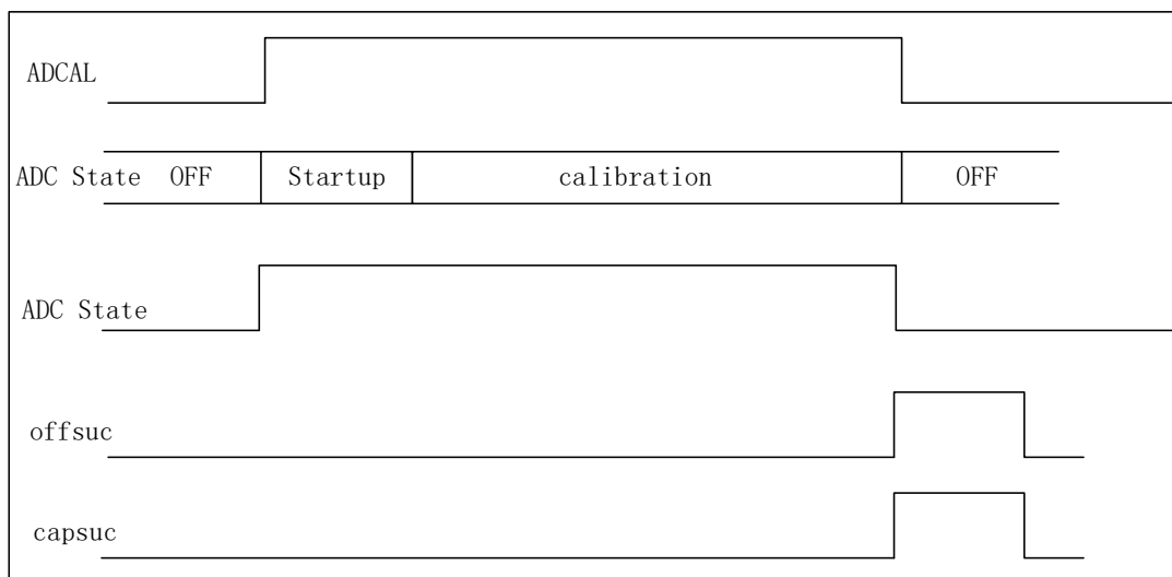
Figure 14-5 ADC Calibration
