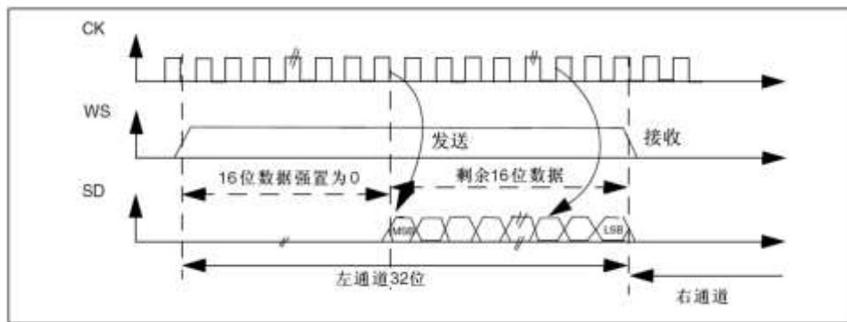
Figure 35-23 LSB aligned 16-bit data extension to 32-bit packet frame, CPOL = 0
