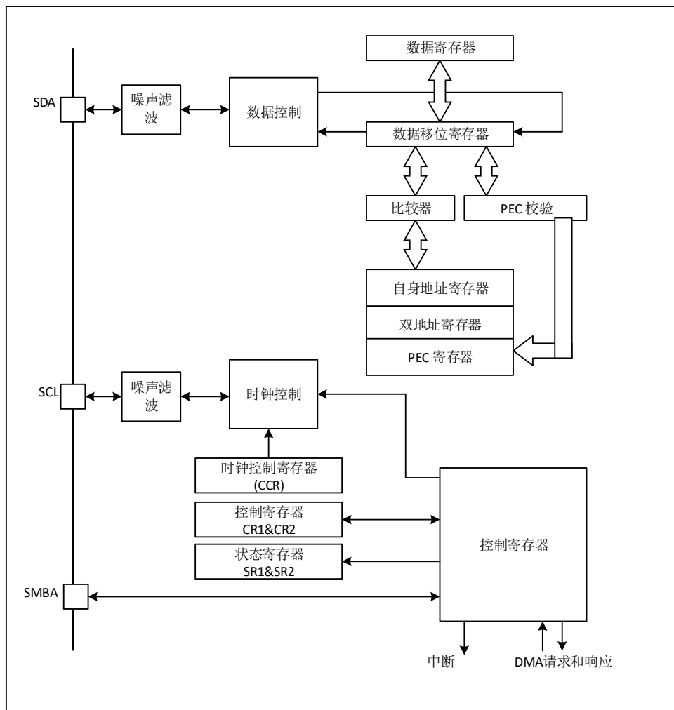
Figure 36-1 I2C Module
