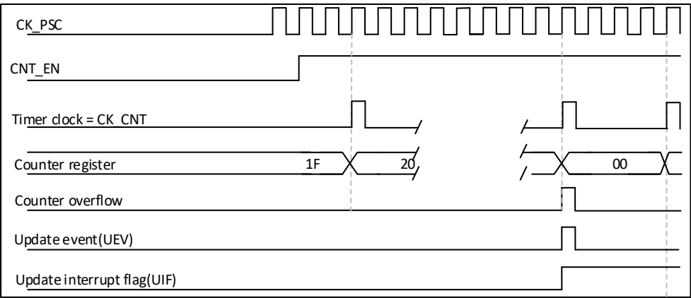
Figure 22-6 Counter timing diagram, internal clock divided by N
