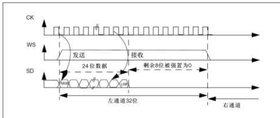
Figure 35-18 MSB aligned 24-bit data, CPKOL = 0
