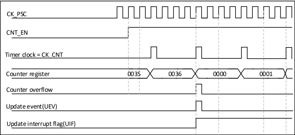
Figure 22-5 Counter timing diagram, internal clock divided by 4
