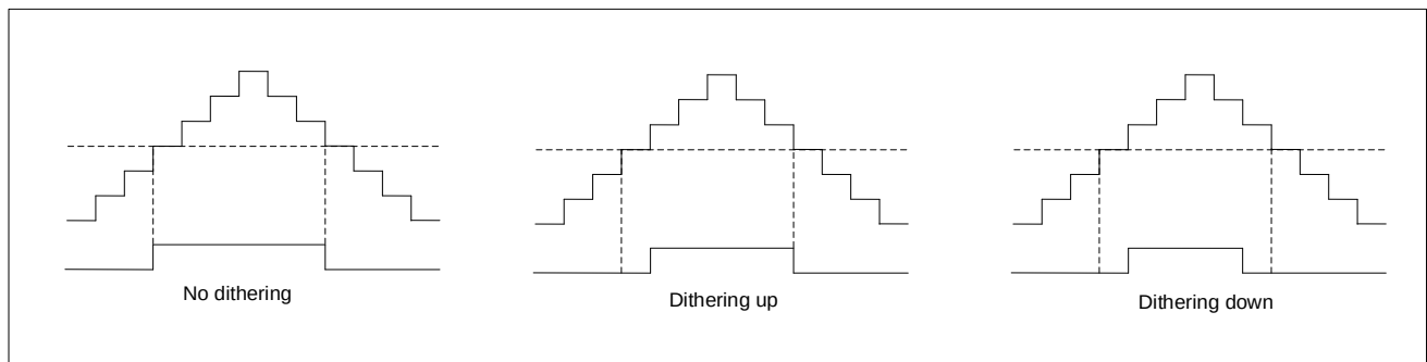
Figure 20-36 Effect of jitter on duty cycle in aligned PWM mode in middle of the figure
