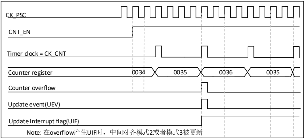
Figure 19-16 Counter timing diagram, internal clock division factor is 4, TIMx_ARR = 0x36
