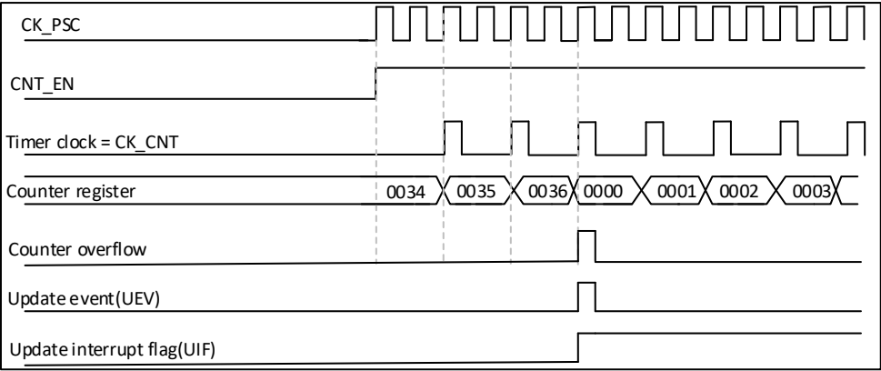
Figure 19-4 Counter timing diagram, internal clock divided by 2
