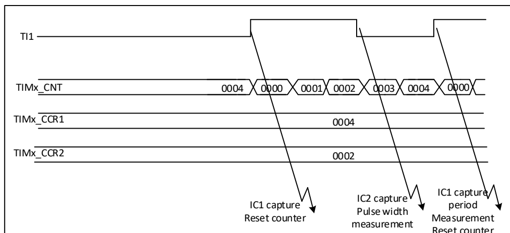
Figure 19-30 PWM input mode timing
