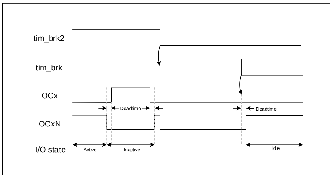
Figure 19-48 PWM output state after braking and braking 2 ( OSSI = 1 )
