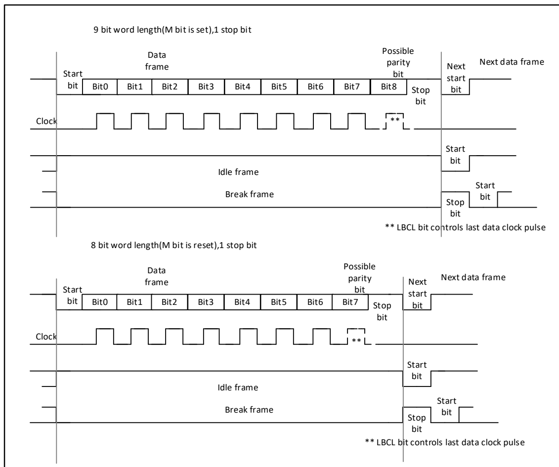
Figure 37-2 word length programming
