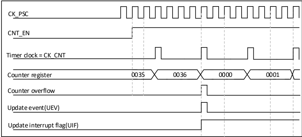
Figure 24-5 Counter timing diagram, internal clock divided by 4
