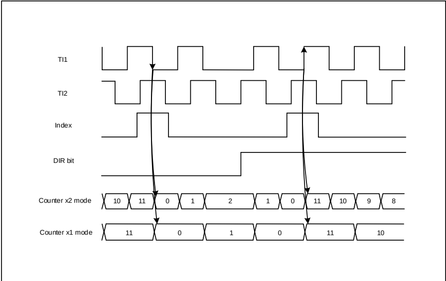
Figure 20-60 IPOS [1: 0] = 01 in x1 and x2 modes
