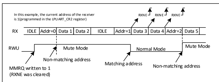
Figure 39-5 Silent mode detected by address flags
