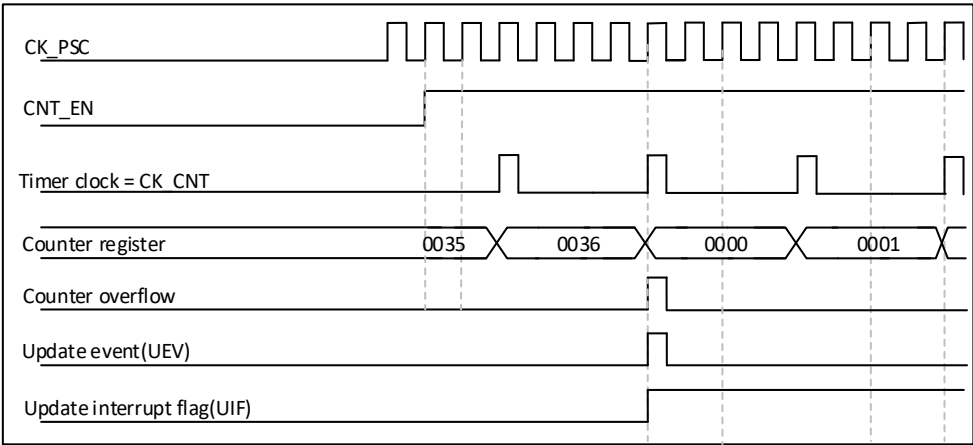
Figure 23-5 Counter timing diagram, internal clock divided by 4
