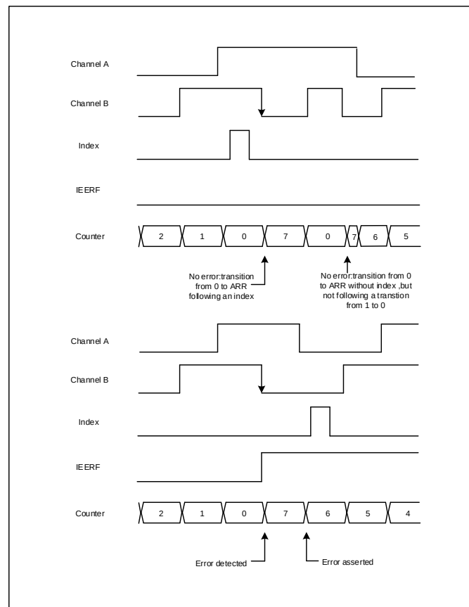
Figure 19-80 Error Detection when Downcoding
