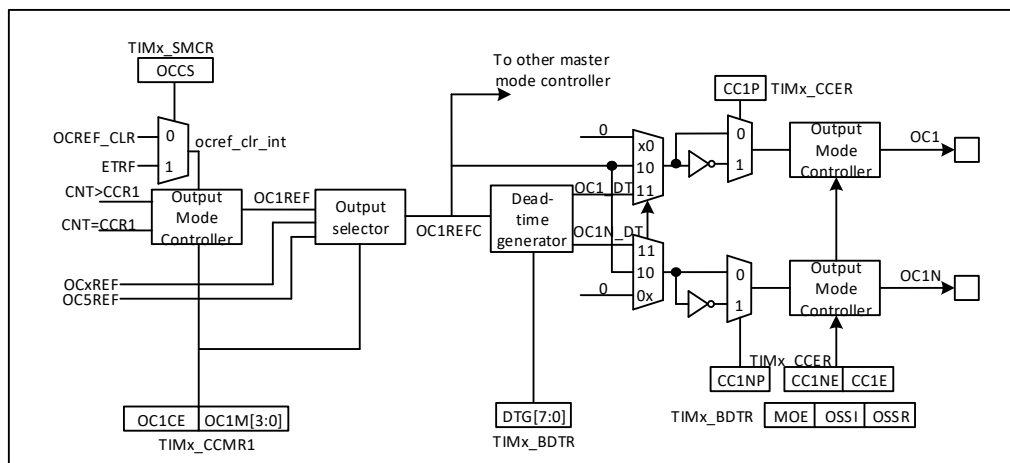
Figure 19-28 Output stage of capture/compare channel (channel 1 to 4)
