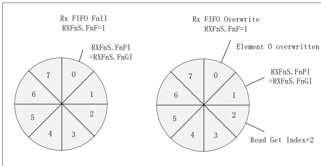
Figure 34-8 Receive FIFO Overflow Processing
