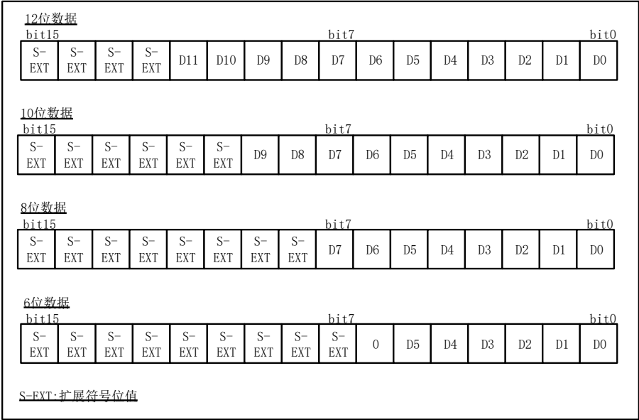
Figure 14-10 right aligned (offset enabled, signed number)
