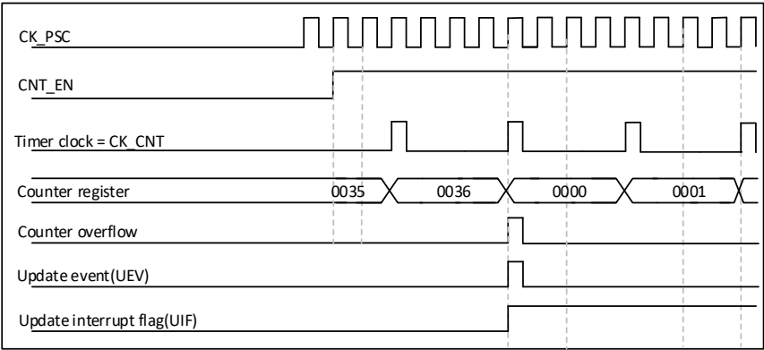
Figure 21-5 Counter timing diagram, internal clock divided by 4
